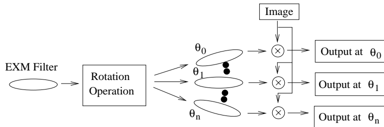
Figure 19: The processing of 3D EXM filtering.
