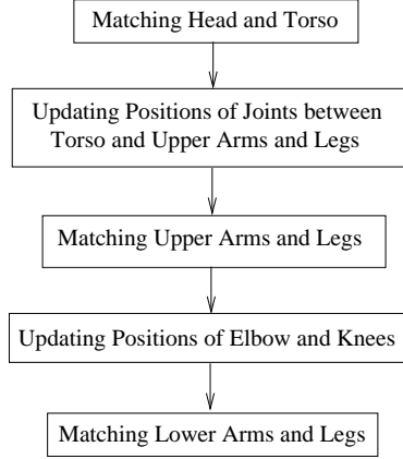
Figure 20: The order of 3D EXM filtering of body parts (top-down).
