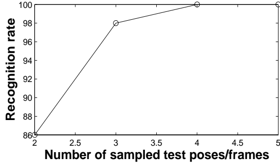
Figure 15: A graph of the recognition rate vs. number of sparse test frames used in the voting. 100%
