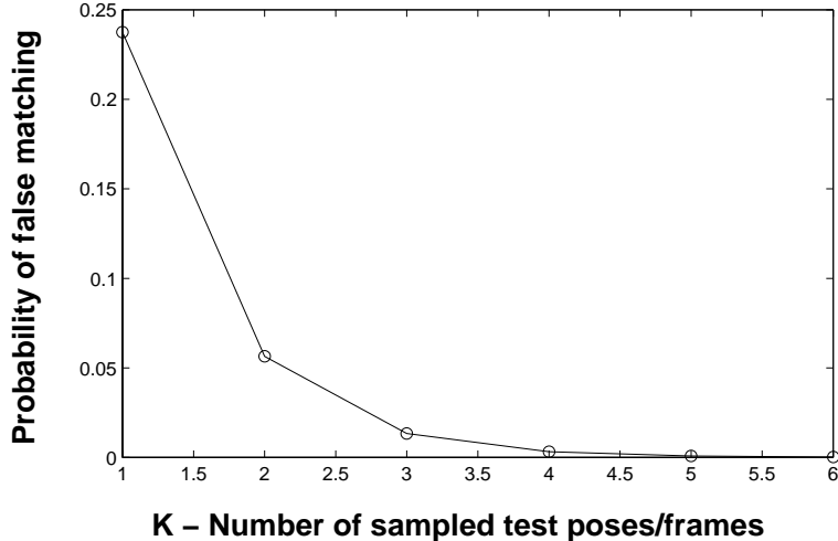
Figure 4: Probability for false matching between jumping and kneeling as a function of K
