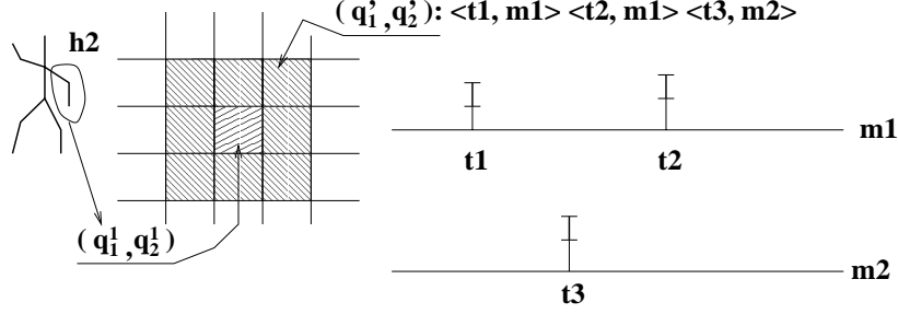
Figure 8: A voting example of the left arm. On the left, the center square (q_1^1, q_2^1) of the grid represents the bin from the pose of the left arm and the surrounding squares are neighboring bins. The upper-right bin (q_1', q_2') contains three entries from models m1 and m2 . These votes are described by the bars on the right diagram. This diagram describes two 1D voting arrays for activity models m1 and m2 .
