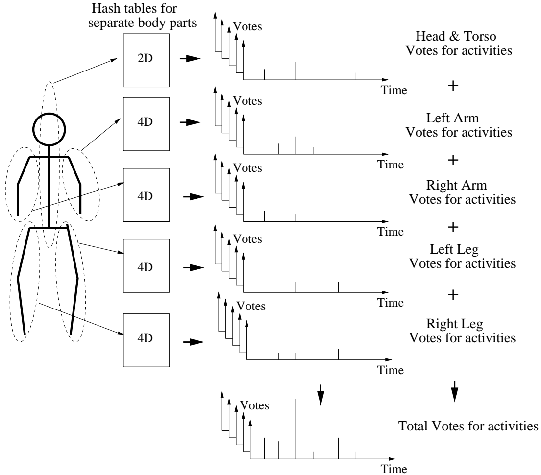
Figure 9: A diagram of the whole voting process which illustrates how voting takes place for the different body parts for different model activities and the way in which the votes for different body parts are combined.
