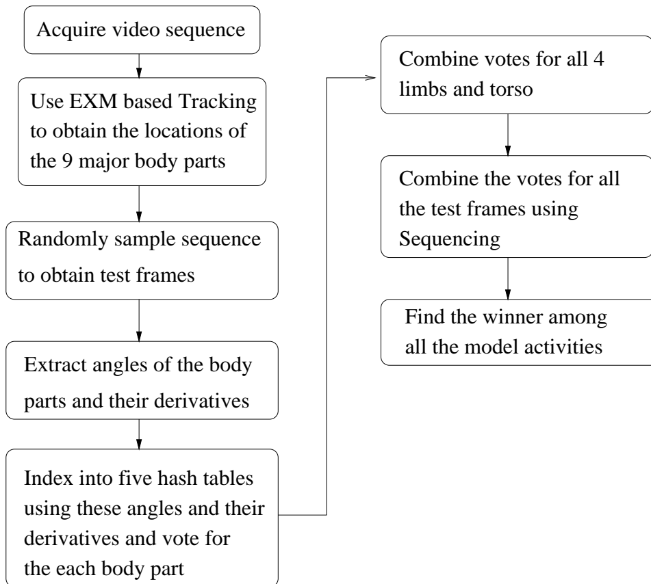
Figure 7: The Flow Diagram of our recognition approach
