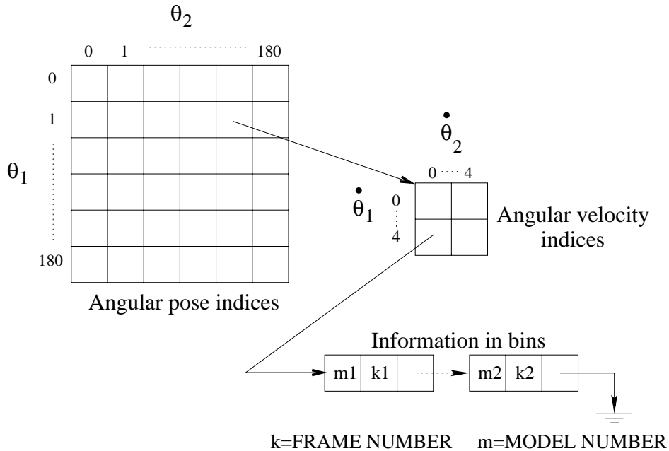
Figure 6: The hash table structure used for the limbs
