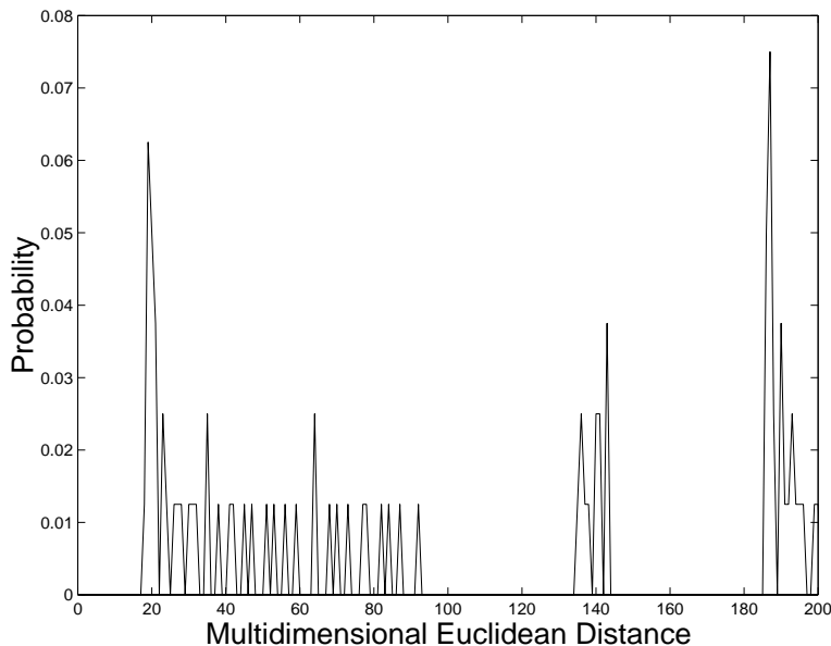
Figure 2: Probability distribution of the multidimensional Euclidean distance for the jumping activity and the sitting activity. This distribution is quite sparse compared to the one in Fig. 3
