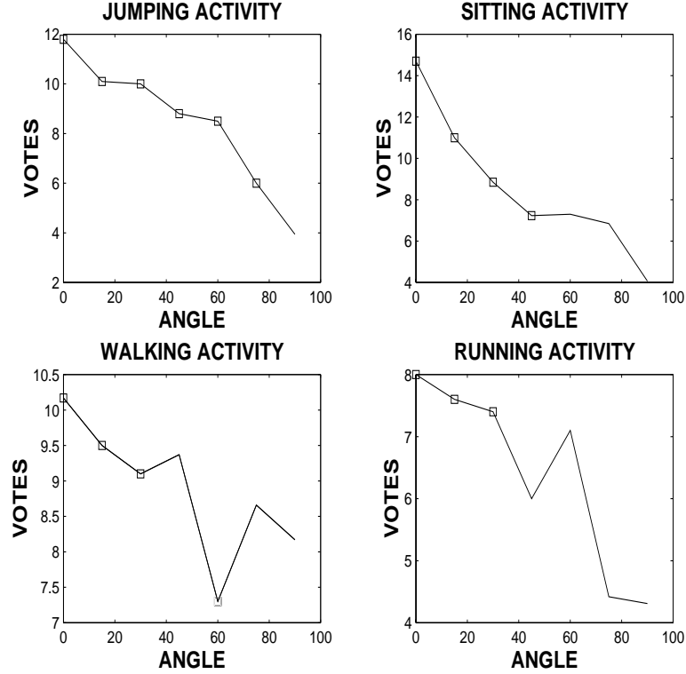
Figure 17: A graph of the votes that were obtained for different view angles of four different activities (Jumping, Sitting, Walking and Running activity). The squares in the graph represent correct recognition of activity. The results show that all the activities were correctly recognized at least up to 30 degrees.
